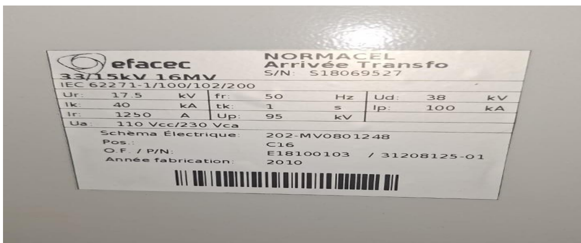
Img5: Plaque signalétique decellule transfo 15kV
